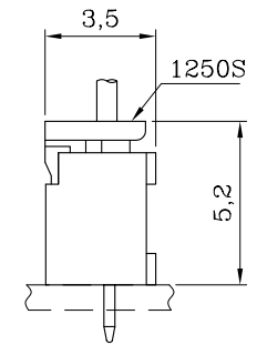
ASSEMBLY LAYOUT
