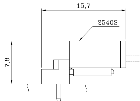
ASSEMBLY LAYOUT
