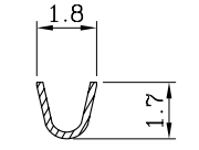
SEC. B-B'
