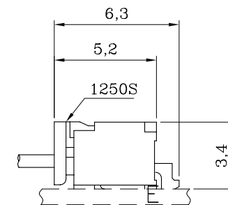
ASSEMBLY LAYOUT
