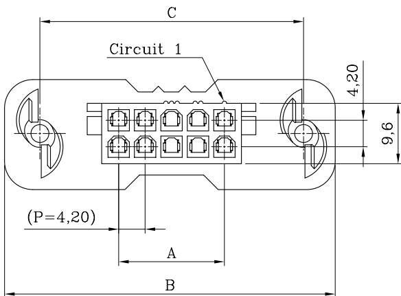
PIN ASSIGNMENT (Bottom View) (SIZE: 3 : 4)
