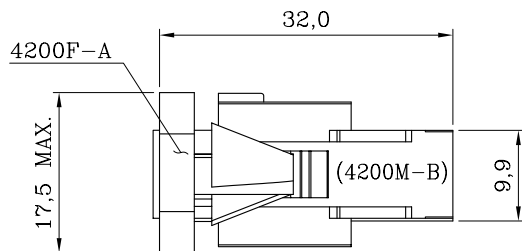
ASSEMBLY VIEW
