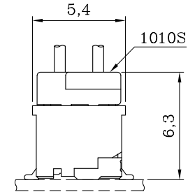
ASSEMBLY LAYOUT
