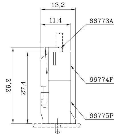
ASSEMBLY LAYOUT
