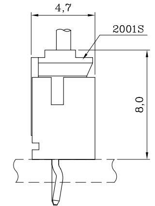
ASSEMBLY LAYOUT
