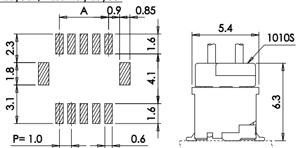
PCB Layout / Assembly Layout
